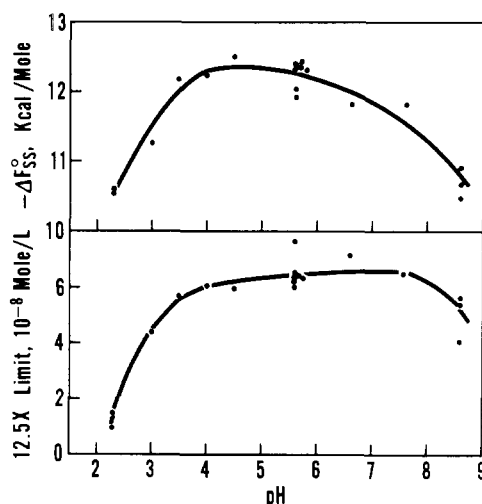
FIGURE 3: Effect of pH on binding energy, -\Delta F_{ss}^\circ , and on cell absorption limit at 12.5×. Cells are from lot W.
