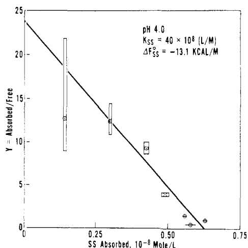
FIGURE 2: Absorption isotherm of 5-Ag on type 21 cells at pH 4.0, 25°. Cell concentration = 3×.
