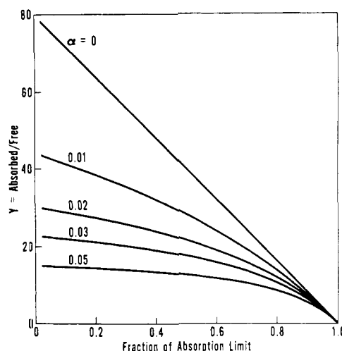
FIGURE 4: Theoretical absorption isotherms for mixtures of active 5-Ag and a fraction, α, of inactive contaminant. K ss L was set at 80.
