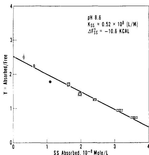
FIGURE 1: Absorption isotherm of 5-Ag on cells of Hansenula wingei type 21, at pH 8.6, 25°. Cell concentration = 12.5×. SS absorbed indicates moles of disulfide absorbed.
